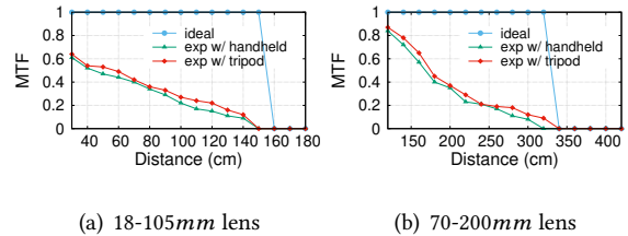
Figure 24: MTF of Nikon D7000 with two lenses.
