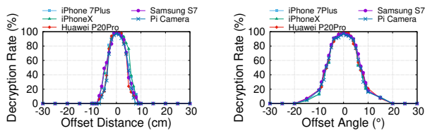
(a) Impact of distance on multi-frame decryption for mQR codes. (b) Impact of angle on multi-frame decryption for mQR codes.
