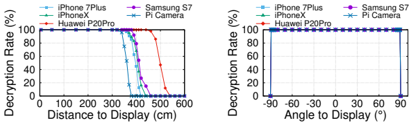
(e) Impact of distance on decoding QR codes in front of the display. (f) Impact of angle on decoding QR codes one meter away from the display.
