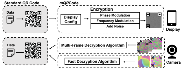
Figure 6: mQRCode system flow.
