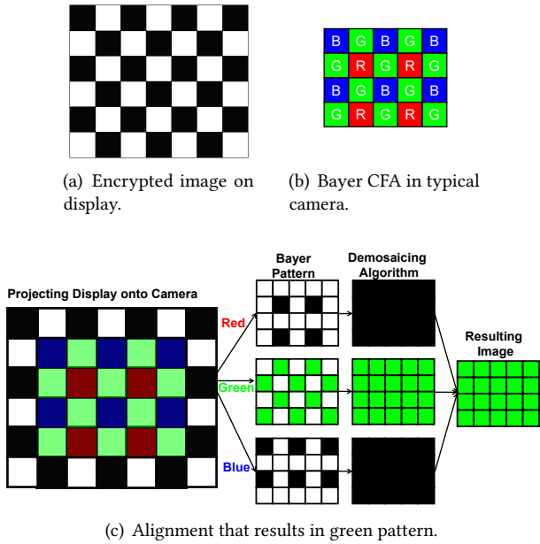
Figure 11: Simulation-based analysis illustrating Moiré patterns in encrypted images.
