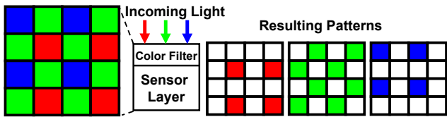
Figure 5: Profile of sensor with the Bayer arrangement of color filters.
