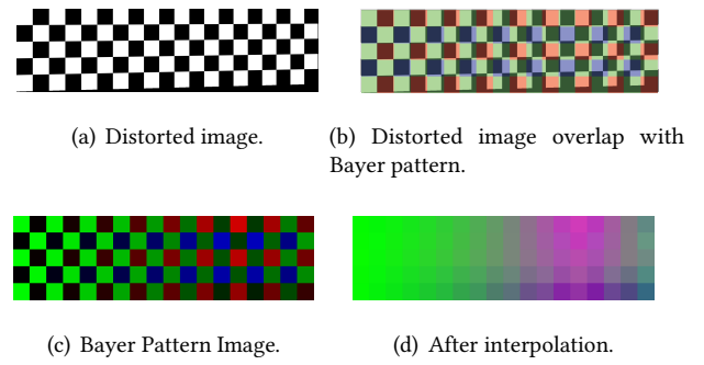
Figure 12: Simulation-based analysis illustrating phase inversion.
